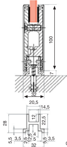
COMET SABİT ALT BAZA DETAYI
